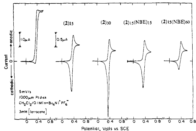
Figure 5. Comparison of the cyclic voltammograms of ferrocene, 2_{15} , 2_{30} , 2_{15}(\text{NBE})_{15} , and 2_{15}(\text{NBE})_{60} in \text{CH}_2\text{Cl}_2/0.1 \text{ M } [n\text{-Bu}_4\text{N}]\text{PF}_6 . The concentration of ferrocene centers is the same (3.0 mM) in each case.
