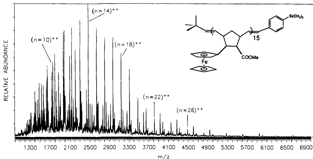
Figure 2. The doubly-charged manifold of peaks in the field desorption mass spectrum of 2_{15} .
