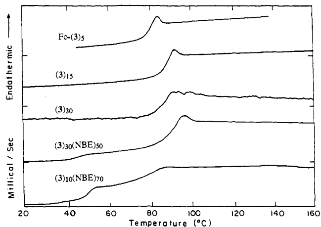
Figure 6. DSC traces of the 3_n polymers and 3_n(\text{NBE})_m block copolymers (scan rate was 20 \text{ }^\circ\text{C}/\text{min} ). The samples were annealed first above the transition temperature for 10 min, and all measurements were repeated several times in order to check reproducibility.
