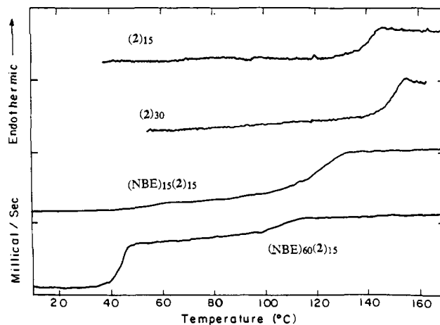
Figure 3. DSC traces of the 2 n polymers and (NBE) n 2 m block copolymers (scan rate 20 °C/min). Samples were annealed first above the transition temperature for 10 min, and all measurements were repeated several times in order to check reproducibility.
