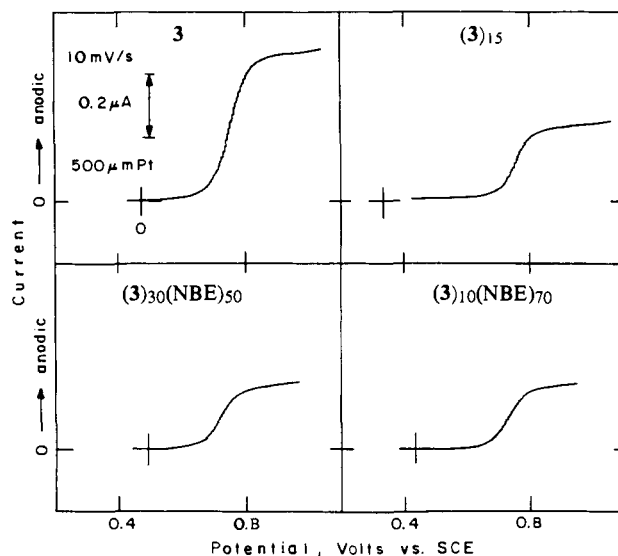
Figure 8. Normal pulse voltammograms of 3, 3 15 , 3 30 (NBE) 50 , and 3 10 (NBE) 70 in CH 2 Cl 2 /0.1 M [n-Bu 4 N]PF 6 . The current was sampled over the last 17 ms of a 57 ms pulse (sweep rate 10 \text{ mV s}^{-1} ; drop time 1 s).
