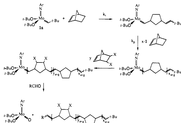
Scheme I. Initiation, Propagation, and Capping Reactions Involved in Preparing Block Copolymers
