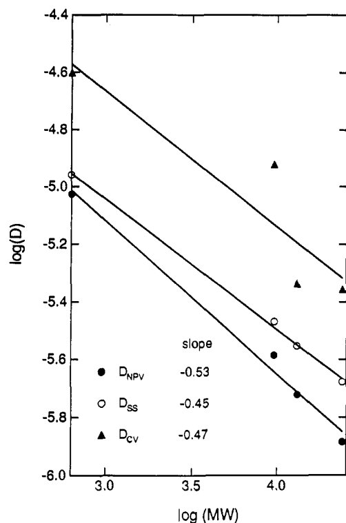
Figure 9. Log-log plot of the diffusion coefficient vs the molecular weight of a series of phenothiazine polymers and a least-squares fit of the data. The diffusion coefficients were obtained experimentally by cyclic voltammetry, steady-state cyclic voltammetry, and normal pulse voltammetry.
