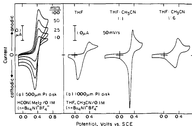
Figure 4. Solvent dependence of the cyclic voltammograms of 2 15 : (a) DMF/0.1 M [ n -Bu 4 N]BF 4 and (b) THF, 1:1 THF/CH 3 CN and 1:6 THF/CH 3 CN. (The supporting electrolyte was 0.1 M [ n -Bu 4 N]BF 4 .)
