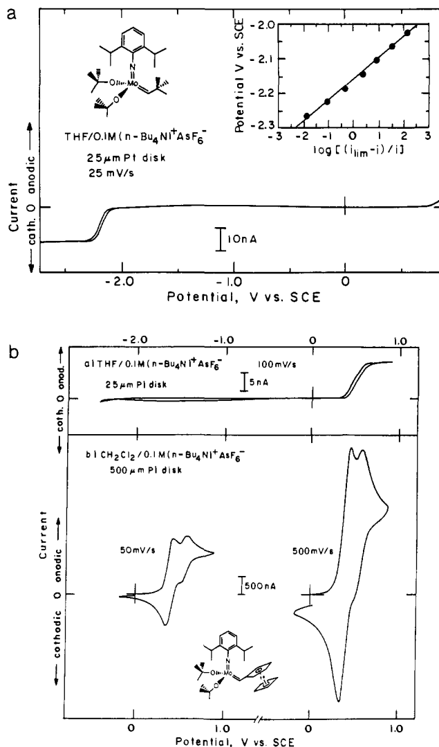
Figure 1. Cyclic voltammetry of (a) 1a in THF/0.1 M [ n -Bu 4 N]AsF 6 at 25 mV s -1 at a 25 \mu m Pt disk electrode and (b) 1b in CH 2 Cl 2 /0.1 M [ n -Bu 4 N]AsF 6 at 50 and 500 mV s -1 at a 500 \mu m Pt disk electrode.
