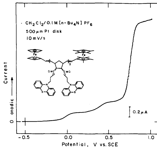
Figure 11. Normal pulse voltammogram of Fc-3 5 -FcMe 8 in CH 2 Cl 2 /0.1 M [n-Bu 4 N]PF 6 . The current was sampled for the last 17 ms of a 57-ms pulse (sweep rate 10 mV s -1 ; drop time 1 s).
